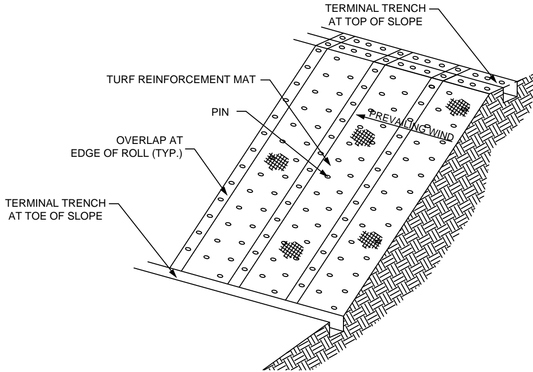
OVERVIEW OF TURF REINFORCEMENT MAT ON A CHANNEL BANK
