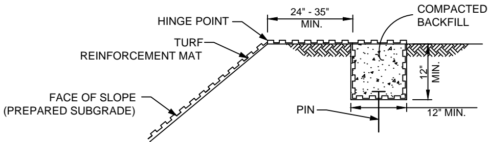
INITIAL TRENCH AT TOP OF SLOPE DETAIL
