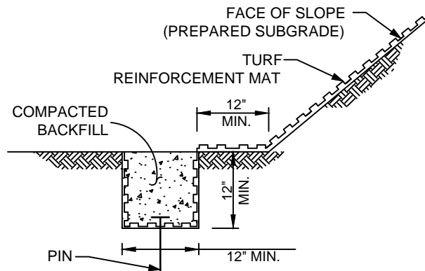
TERMINAL TRENCH AT TOE OF SLOPE DETAIL
