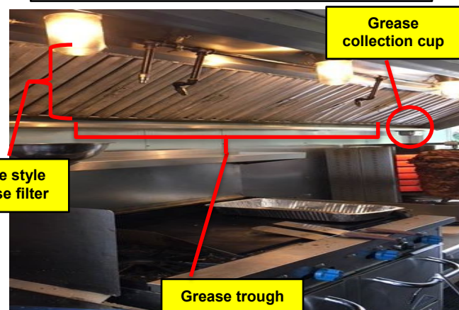
Type I hood over grease producing cooking equipment
