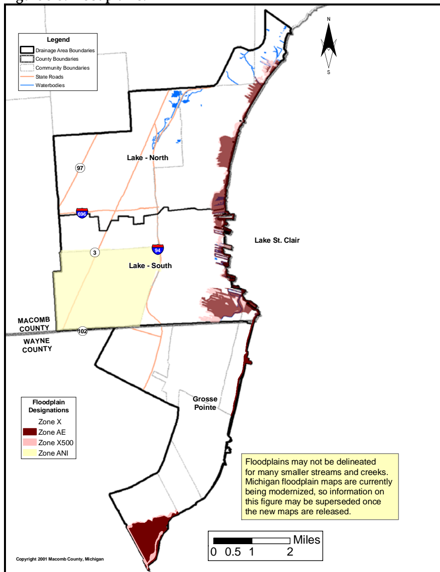
Figure 3-3. Floodplains.
