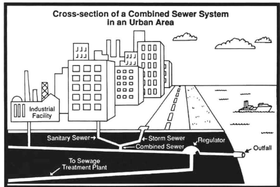
Figure 2-11. Schematic of a combined sewer system.
